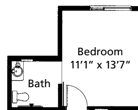
Plan MC (Memory Care) 218 sq.ft.
