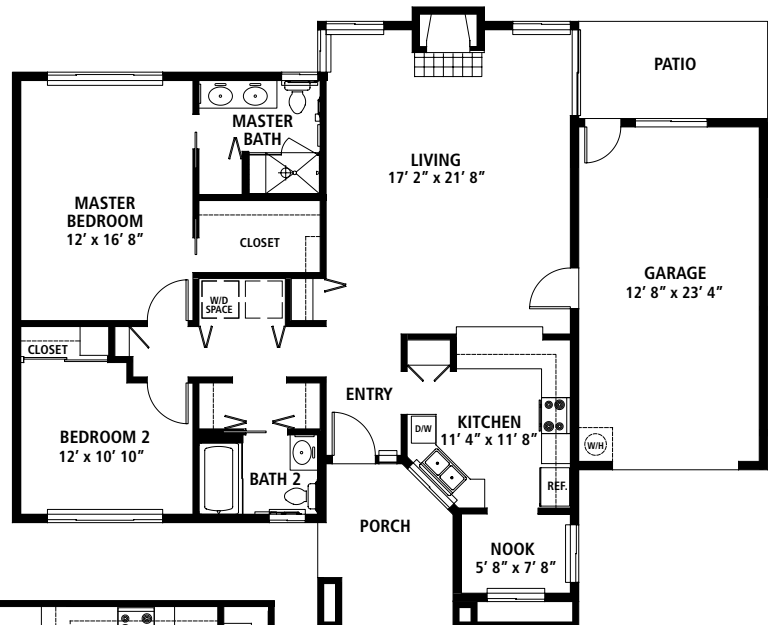
COTTAGE LN Two Bedrooms 1299 sq. ft.
