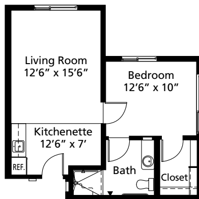
Plan D (Assisted Living) 585 sq.ft.
