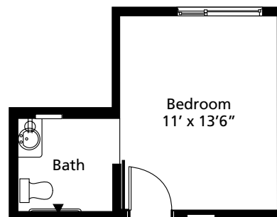
Plan MC (Memory Care) 218 sq.ft.
