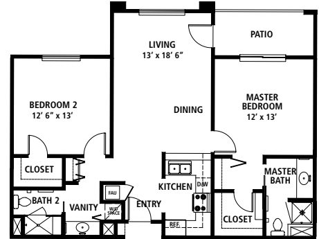
APT F Two Bedrooms 1014 sq. ft.
